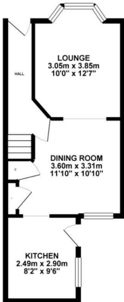
GROUND FLOOR 34.56 sq. m. ( 372.00 sq. ft. )
